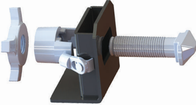
SOMUN LOCKING NUT
